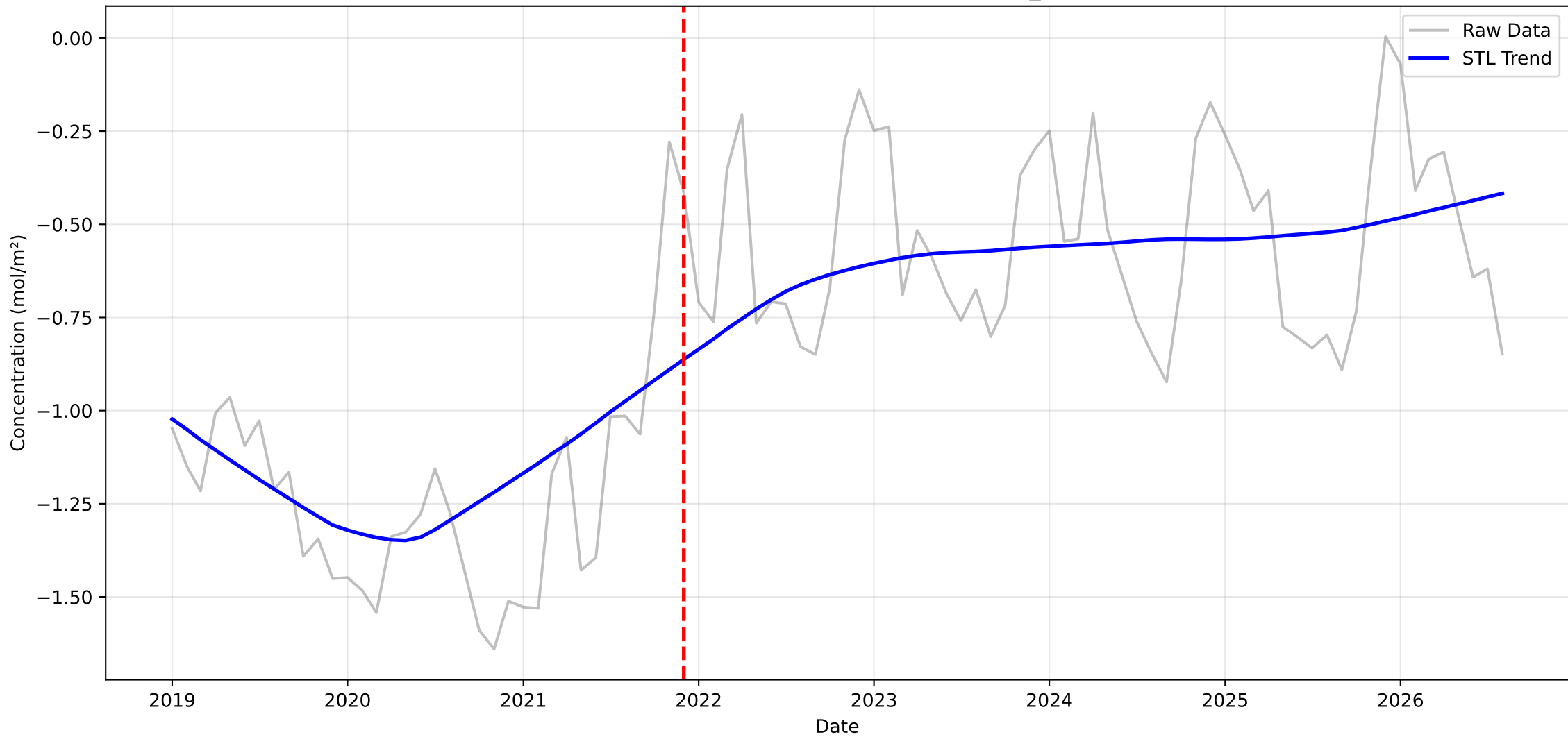
Structural Breakpoint Analysis: UVAI in Middle_Mountains
