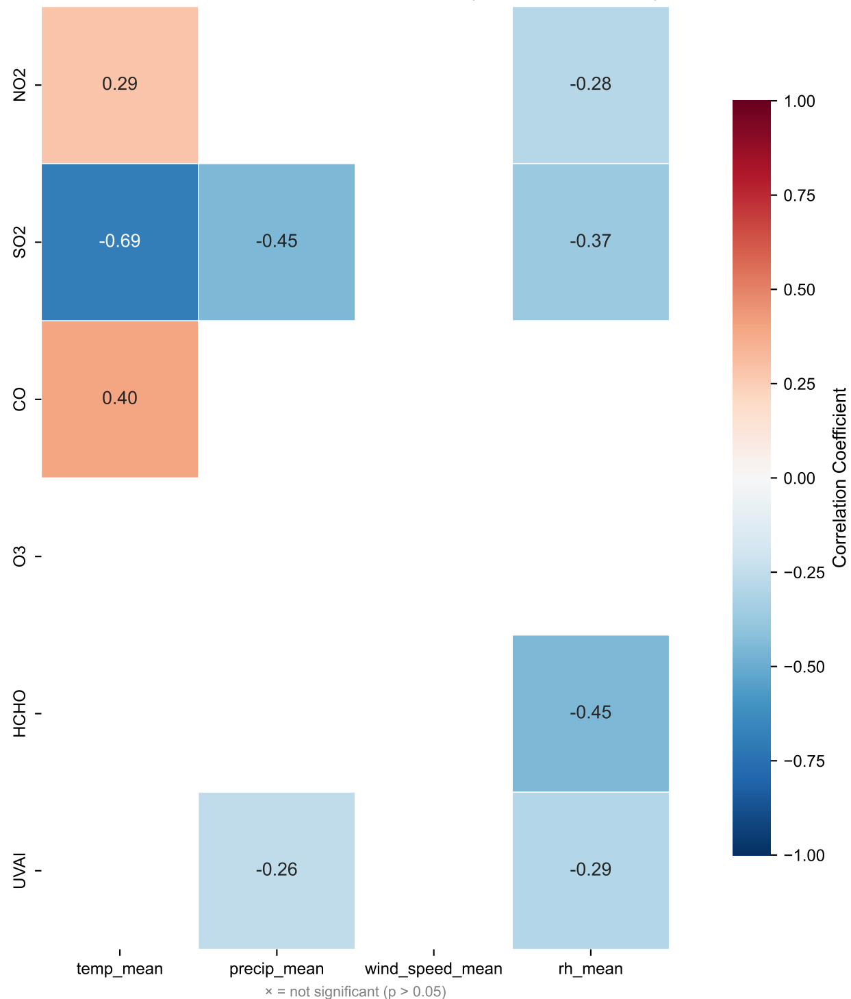
Pearson Correlation: Pollutants vs Climate (Middle_Mountains)
