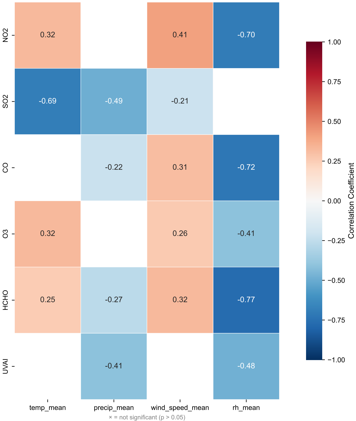
Pearson Correlation: Pollutants vs Climate (Siwalik)
