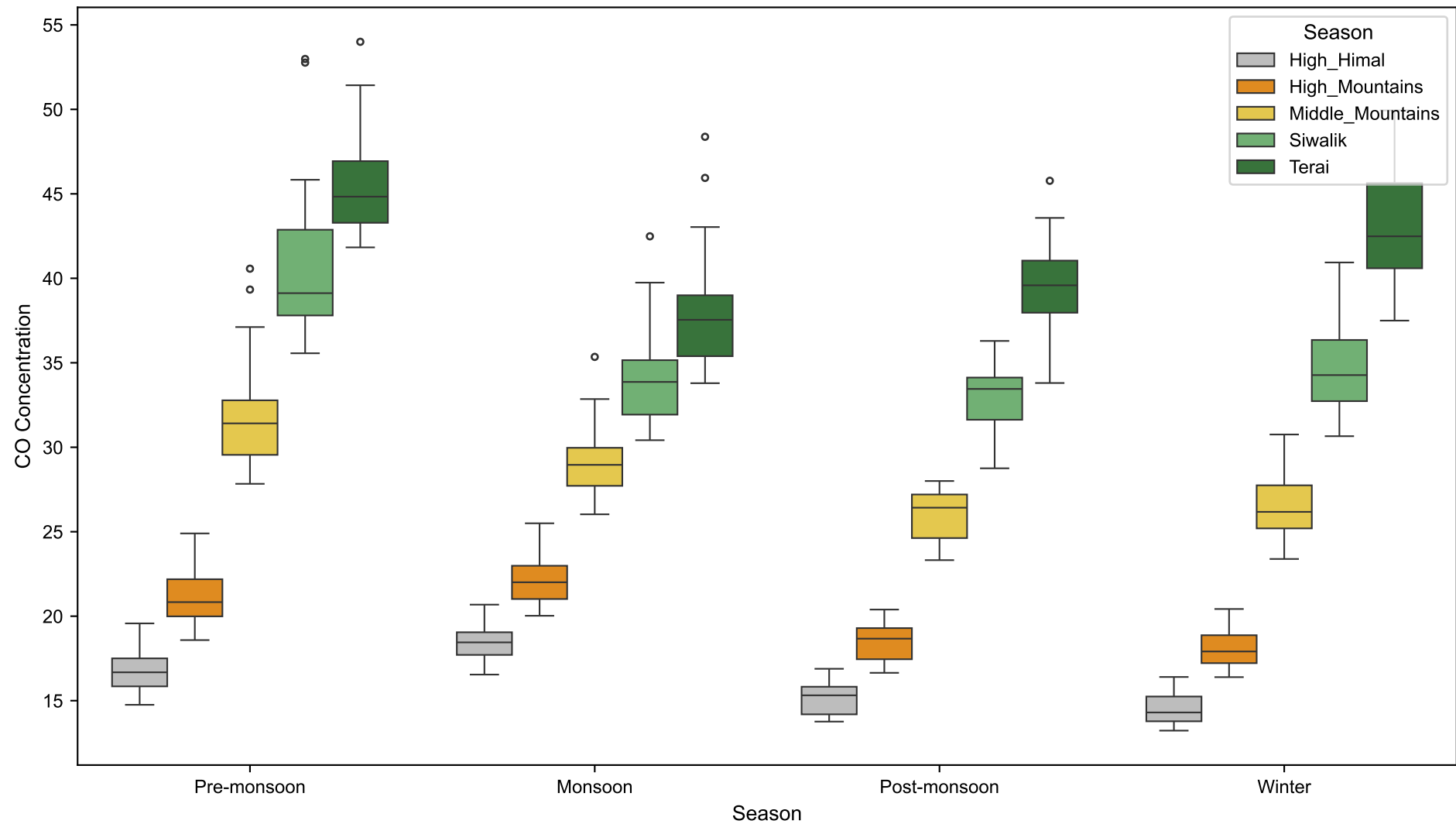
Seasonal Carbon Monoxide Distribution
