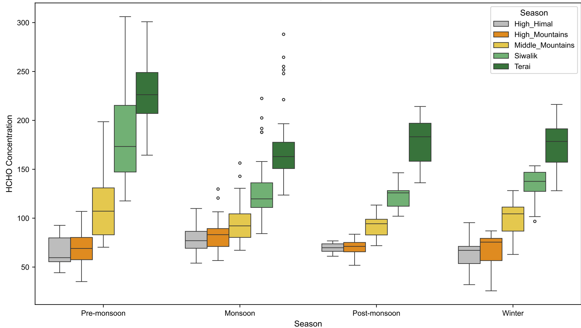
Seasonal Formaldehyde Distribution
