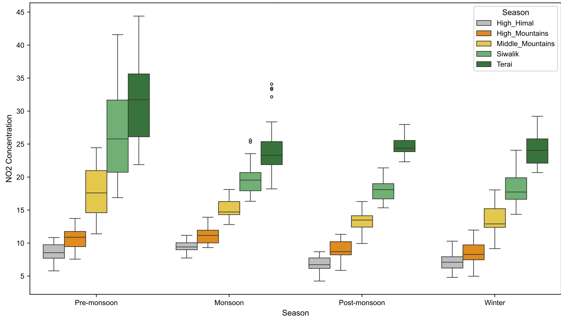
Seasonal Nitrogen Dioxide Distribution
