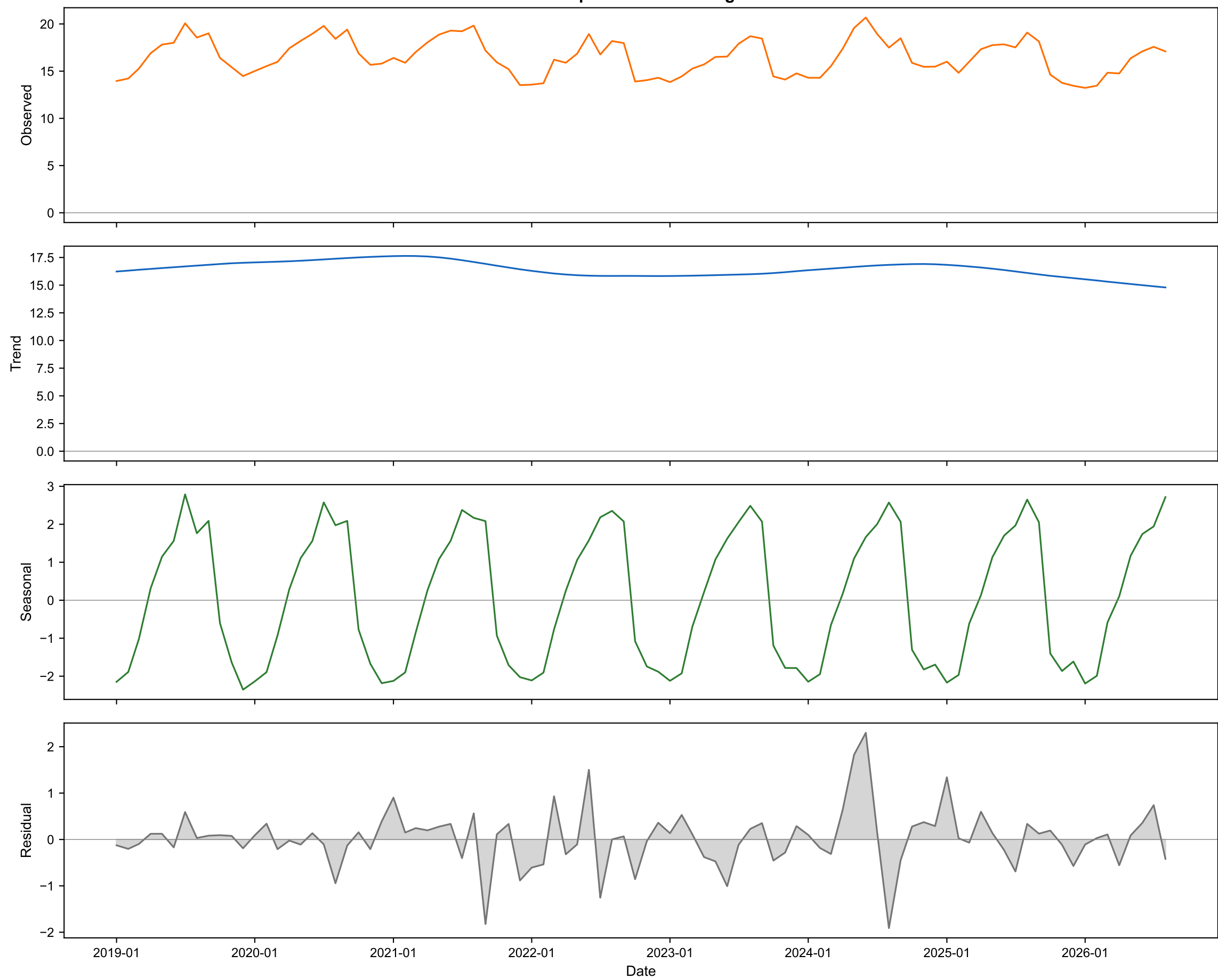
STL Decomposition: CO — High Himal
