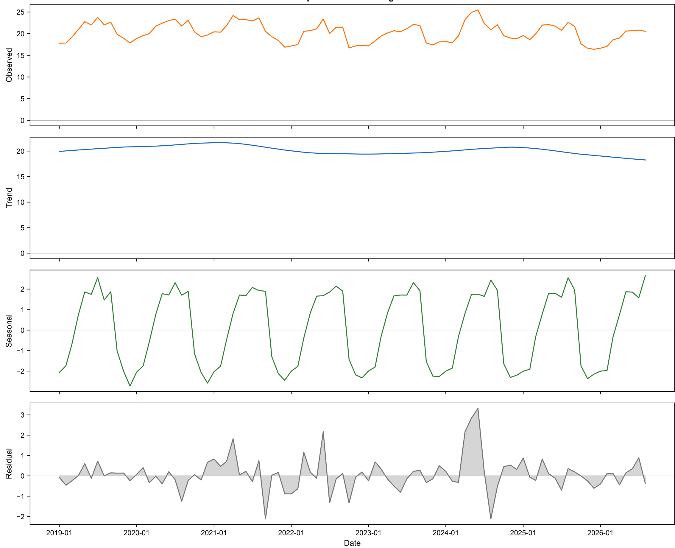
STL Decomposition: CO — High Mountains
