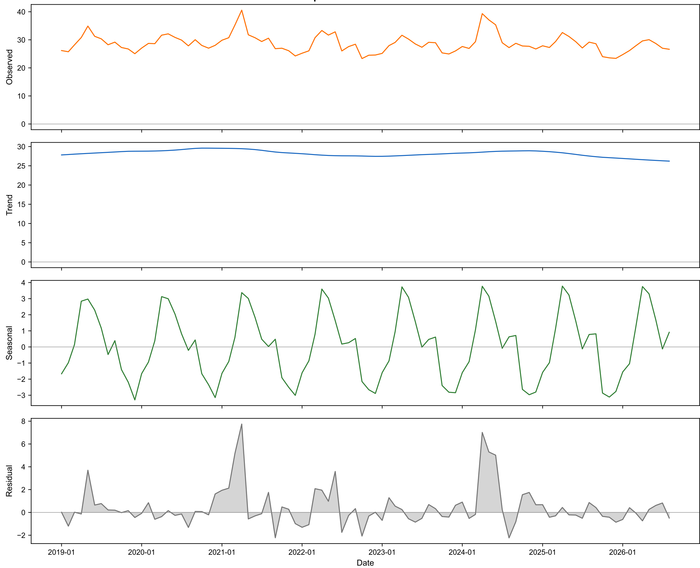
STL Decomposition: CO — Middle Mountains
