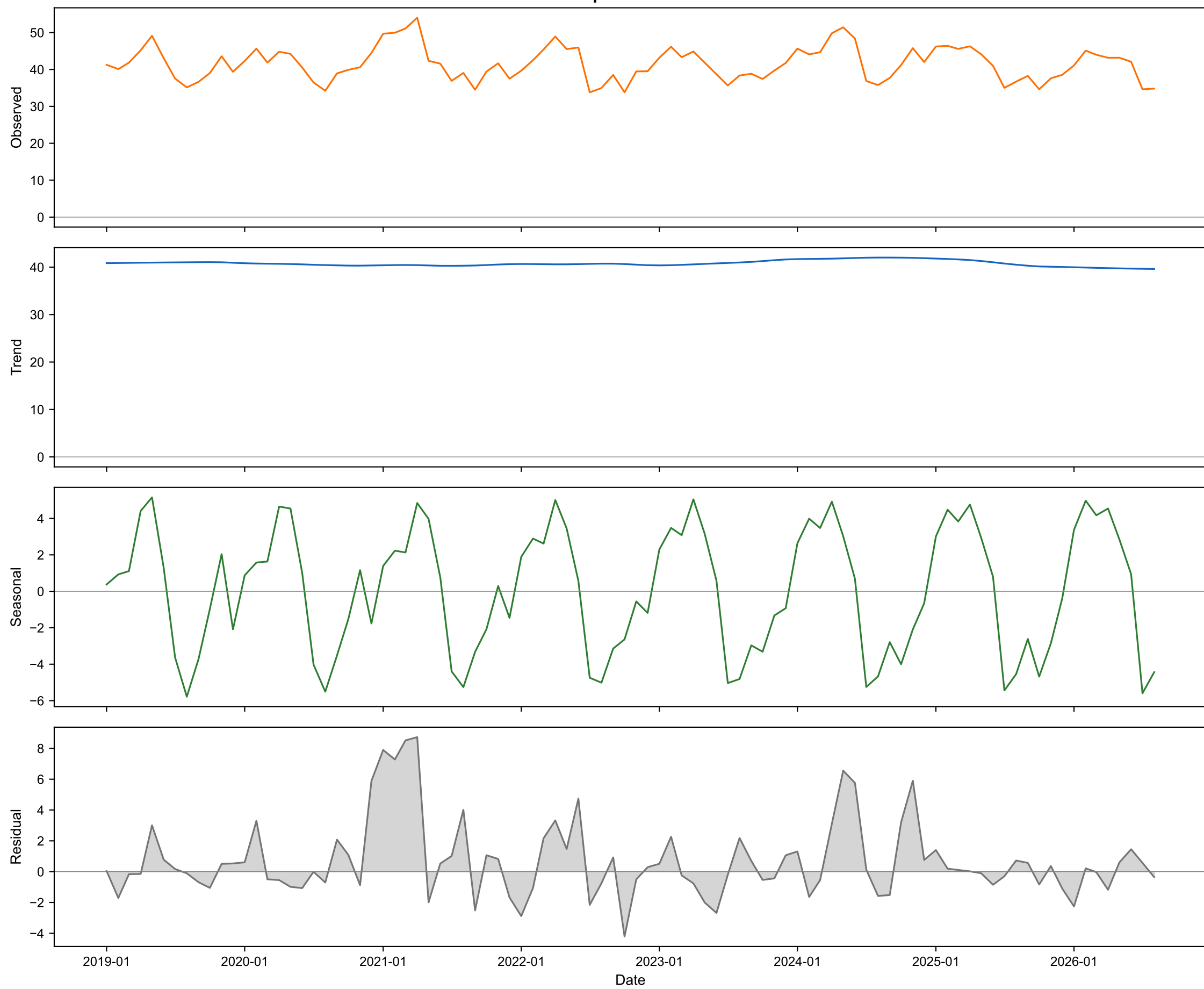
STL Decomposition: CO — Terai
