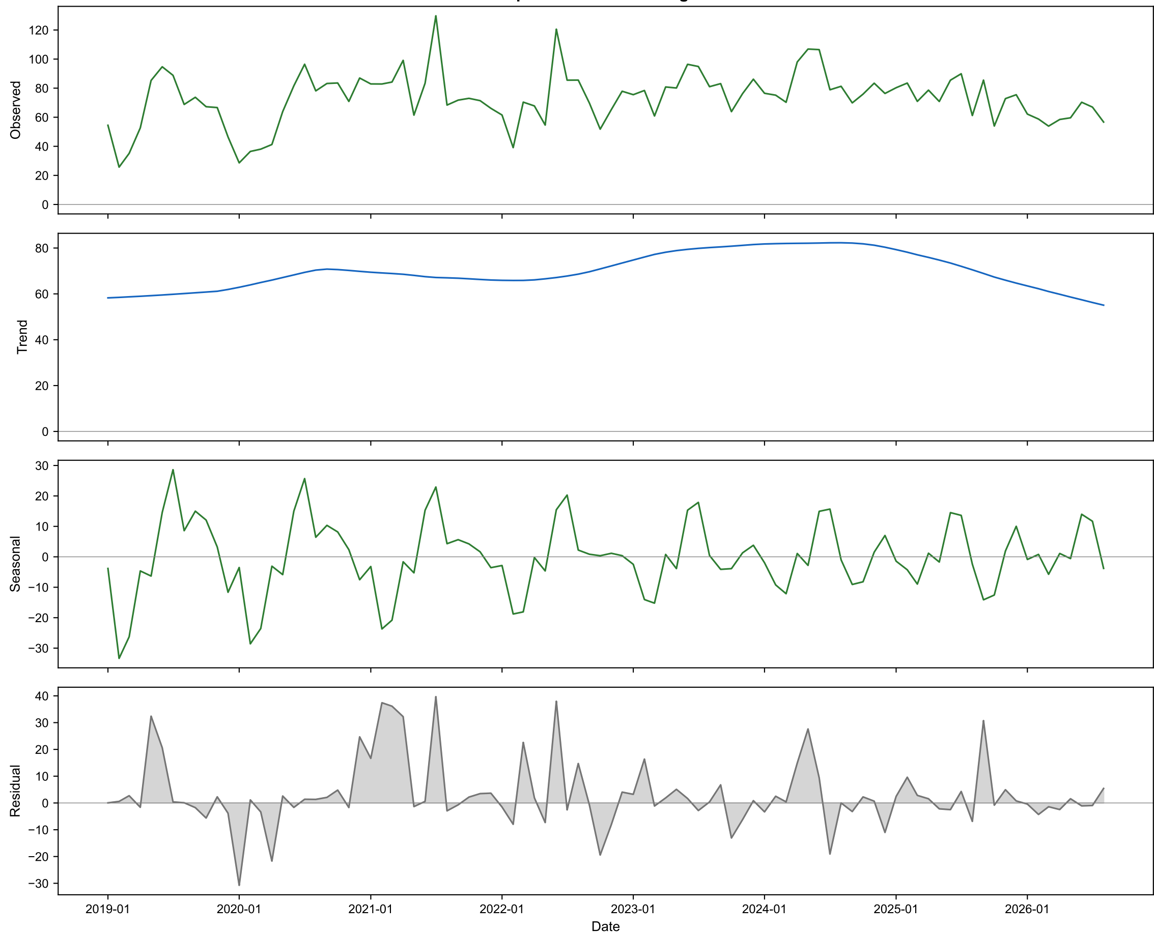
STL Decomposition: HCHO — High Mountains
