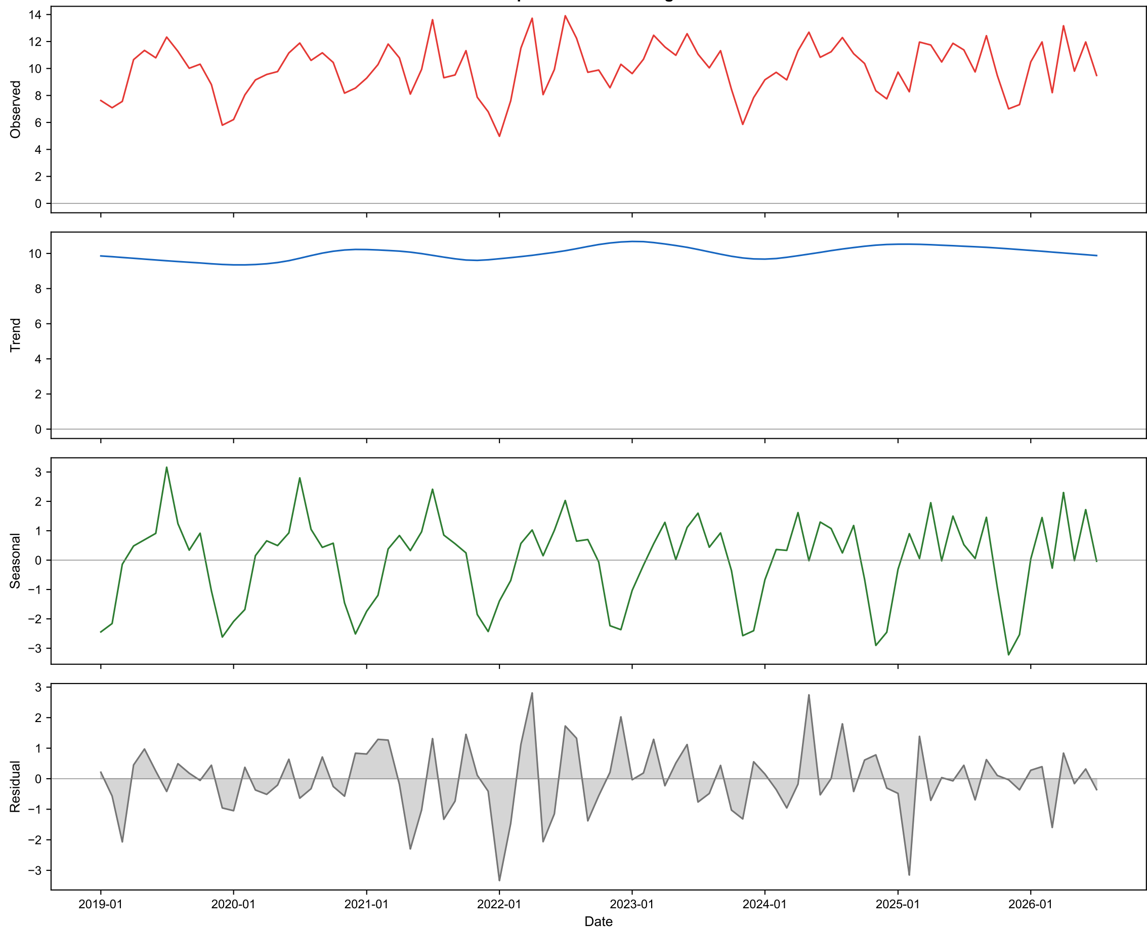
STL Decomposition: NO2 — High Mountains
