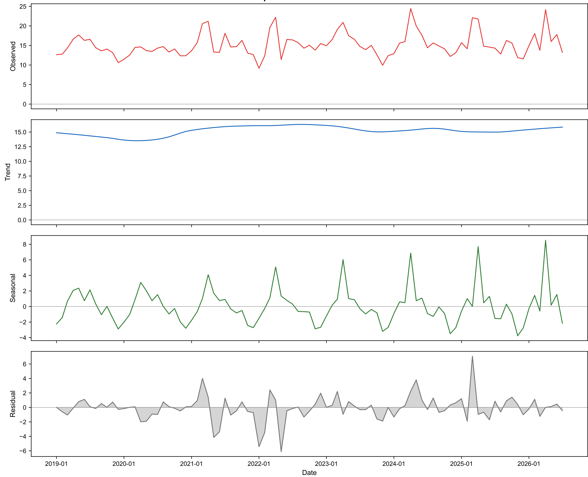
STL Decomposition: NO2 — Middle Mountains
