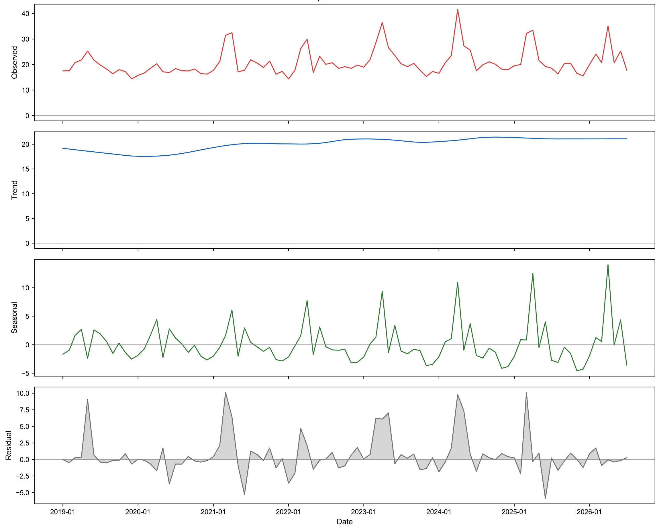
STL Decomposition: NO2 — Siwalik
