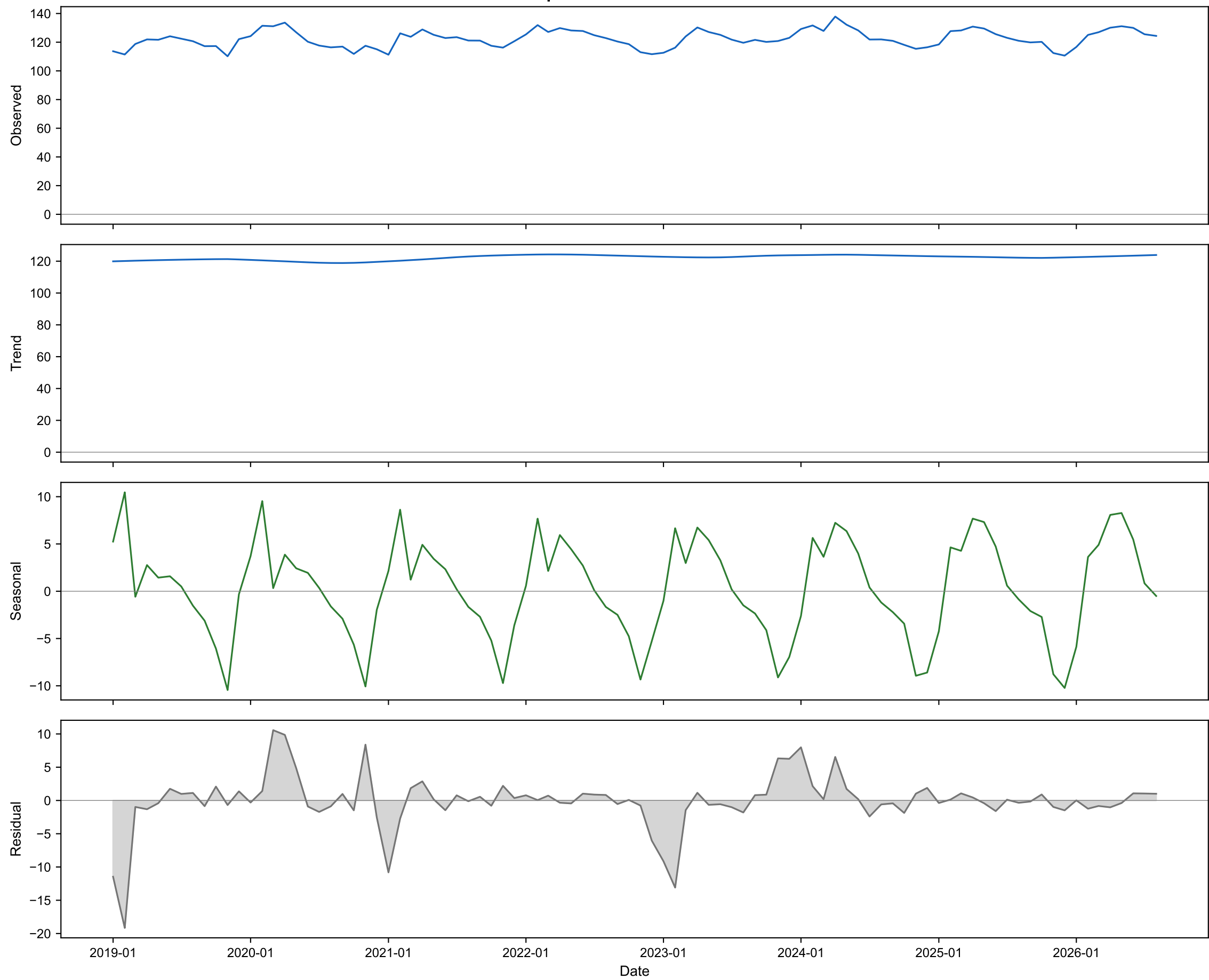
STL Decomposition: O3 — Middle Mountains
