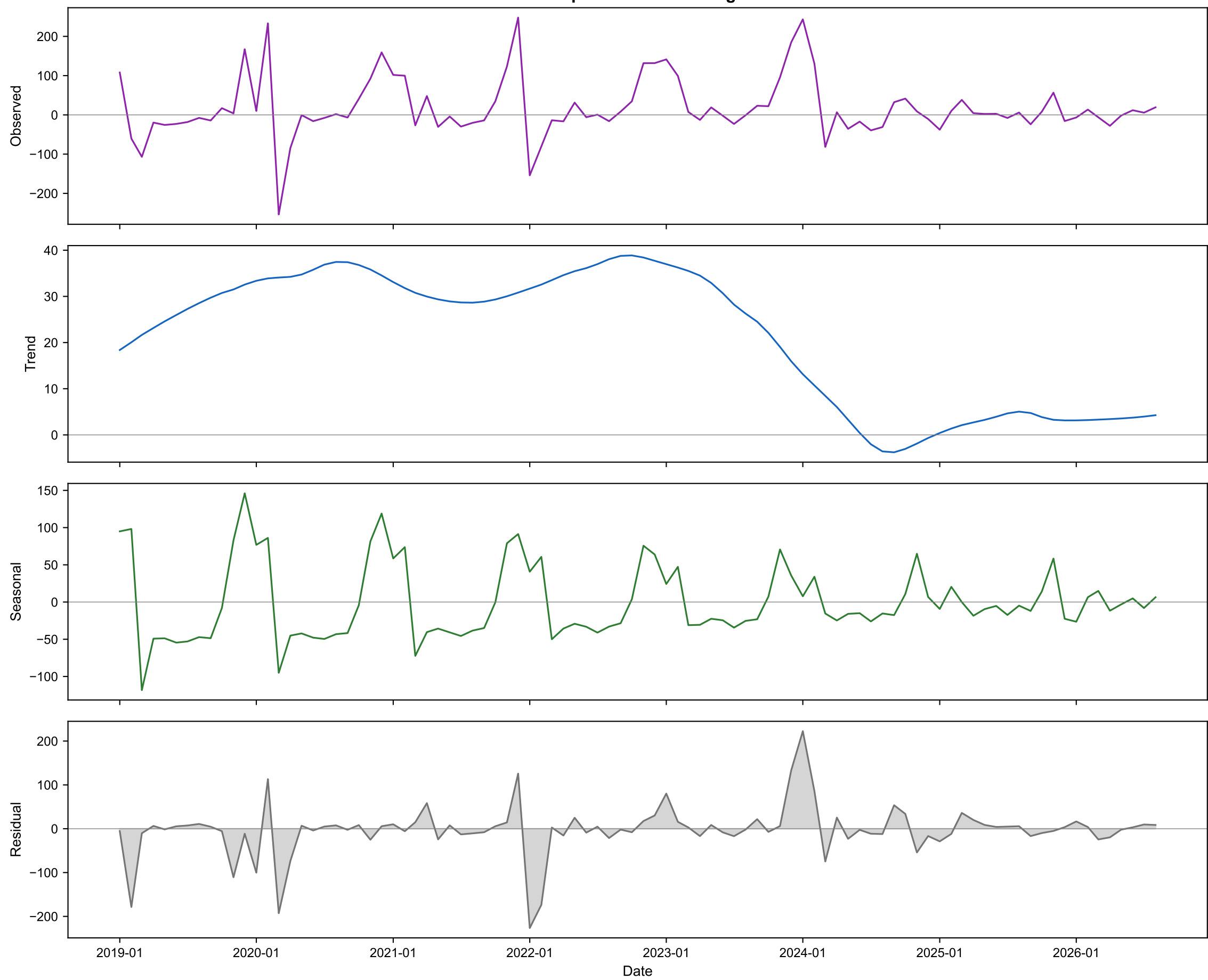
STL Decomposition: SO2 — High Himal
