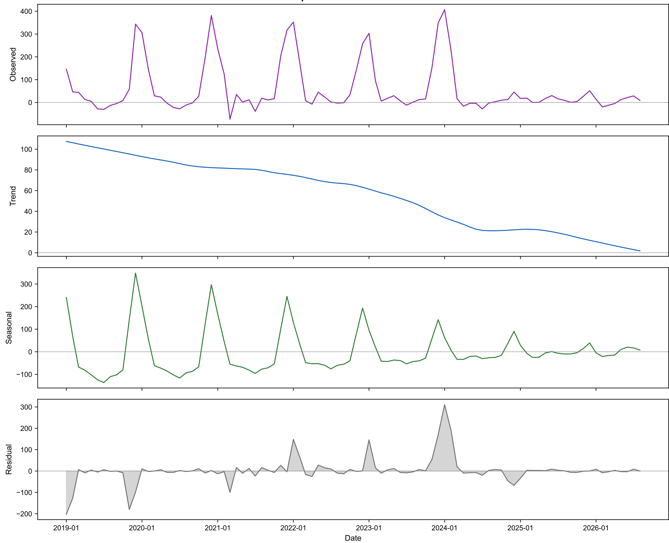
STL Decomposition: SO2 — Middle Mountains
