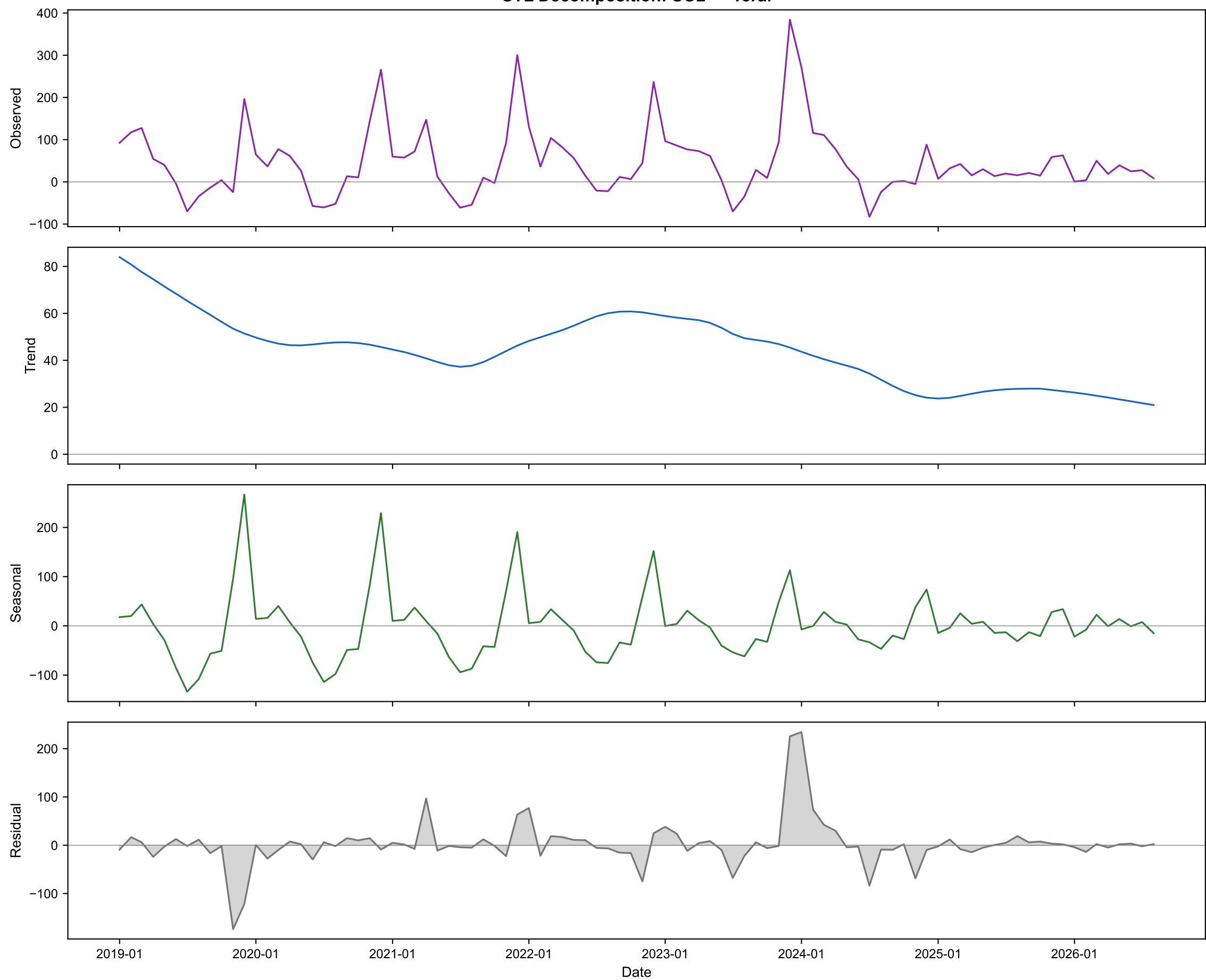
STL Decomposition: SO2 — Terai
