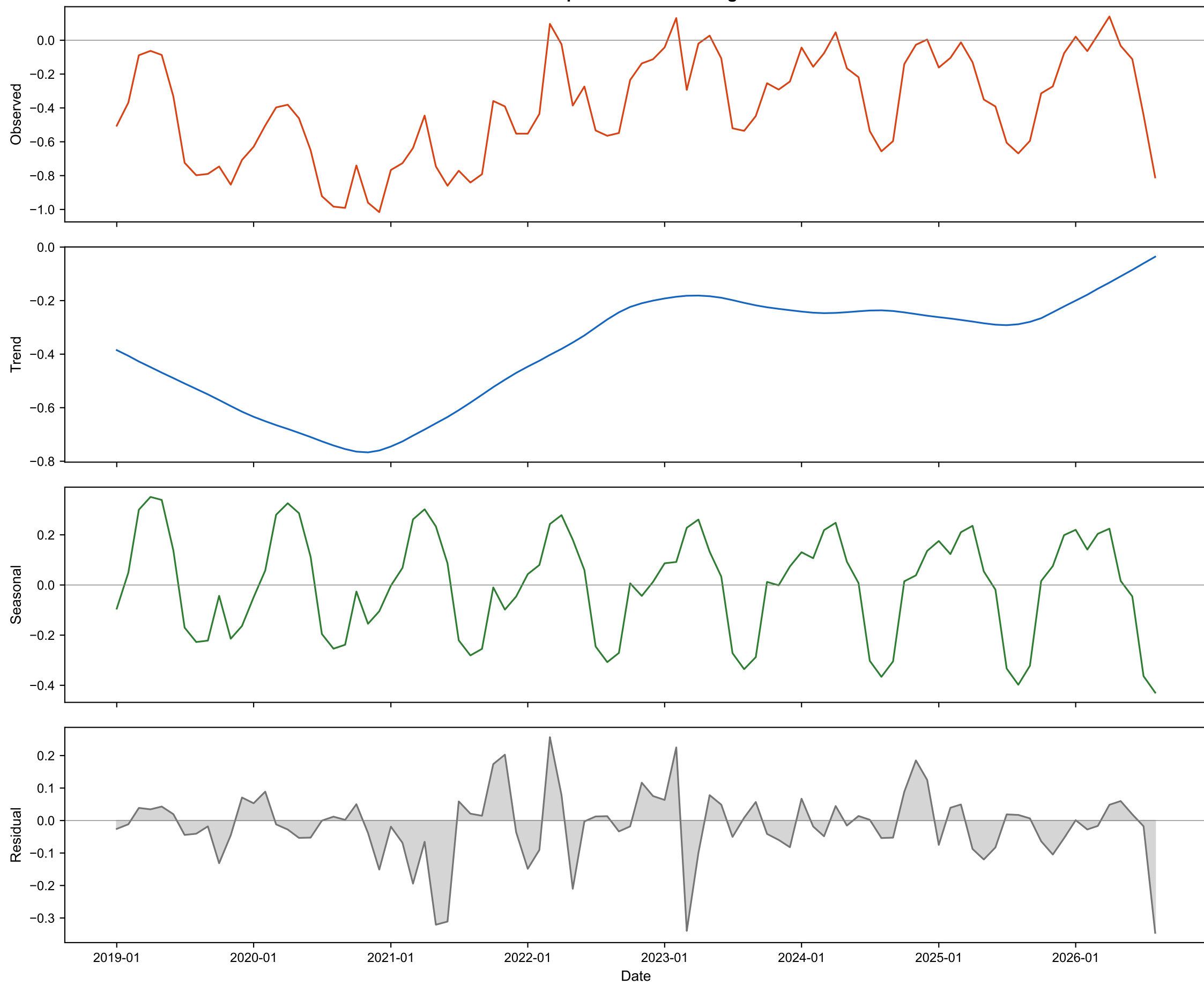
STL Decomposition: UVAI — High Himal
