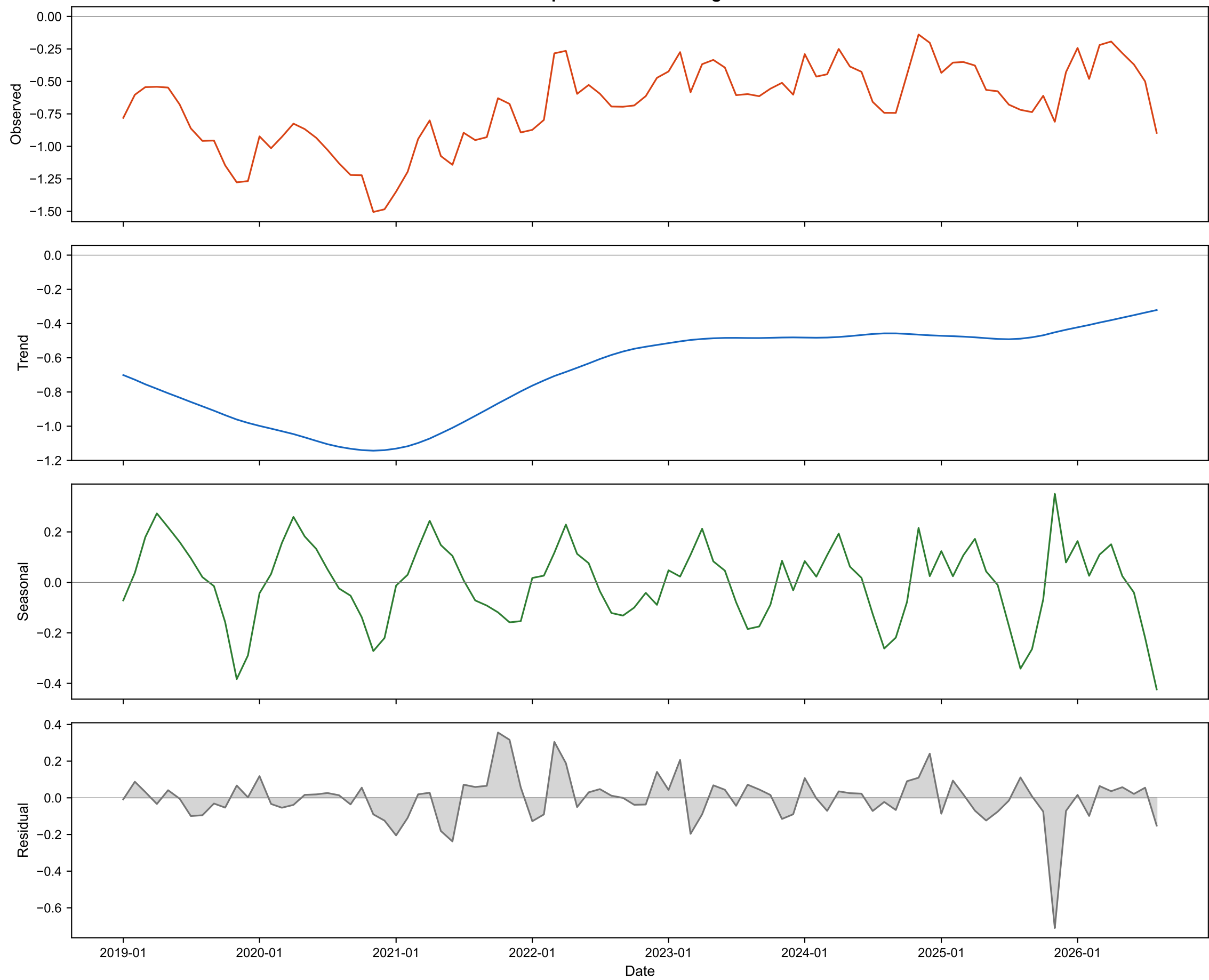
STL Decomposition: UVAI — High Mountains
