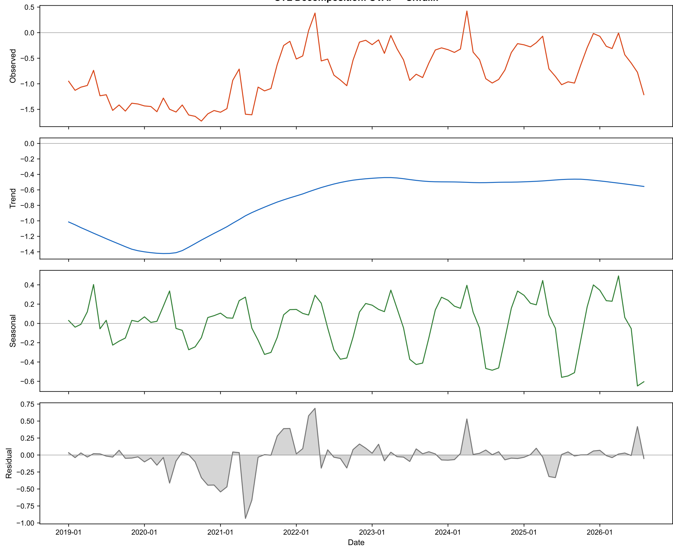
STL Decomposition: UVAI — Siwalik
