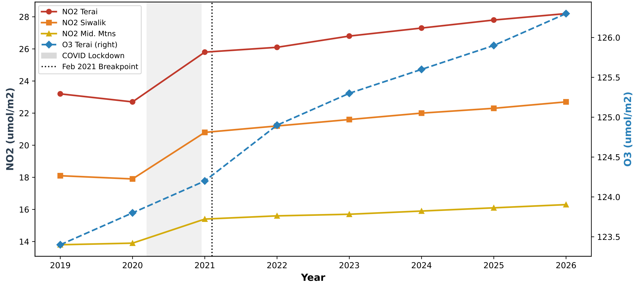
Figure 2 — Annual Mean NO2 and O3 Trends by Physiographic Zone (2019-2026) (Sentinel-5P TROPOMI; shaded = COVID-19 lockdown; dotted line = Feb 2021 Breakpoint)
