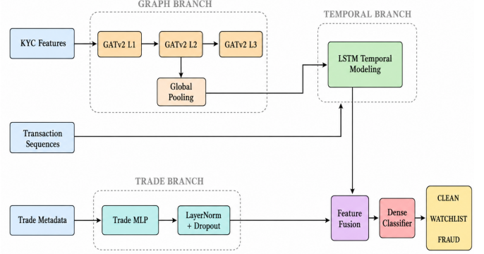
Fig. 5: Hybrid multi-modal graph-learning architecture integrating GATv2-based structural neighborhood propagation, temporal LSTM behavioral modeling, and trade-feature fusion for intelligent TBML detection.
