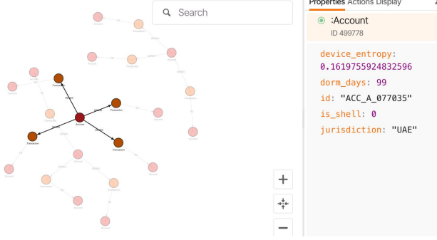
Fig. 4: Memgraph-based heterogeneous financial graph visualization showing interconnected account and transaction entities with multi-hop transactional relationships used for localized TBML subgraph extraction and graph-learning inference.
