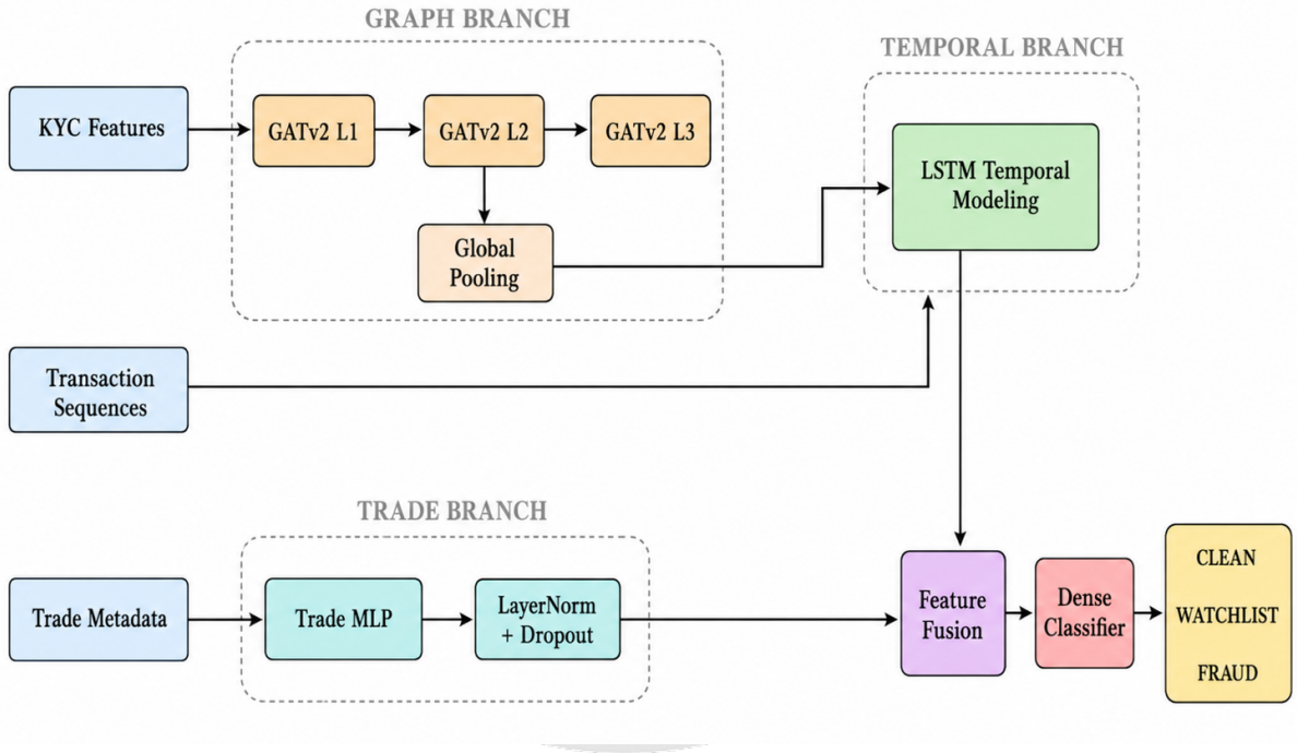
Figure 5.3: Architecture of the Proposed Hybrid HGNN–LSTM Fraud Detection Module
