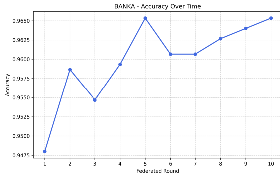
(a) BANKA Accuracy vs Federated Aggregation Rounds
