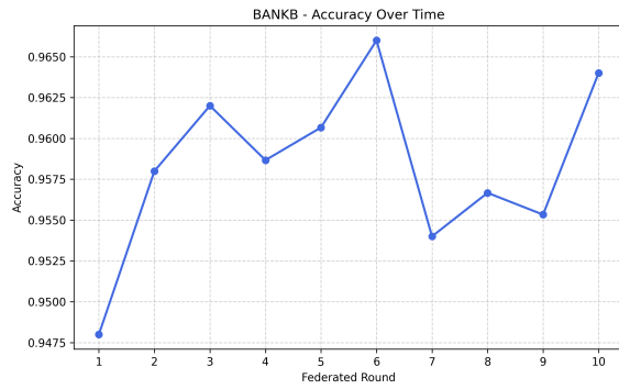
(a) BANKB Accuracy vs Federated Aggregation Rounds
