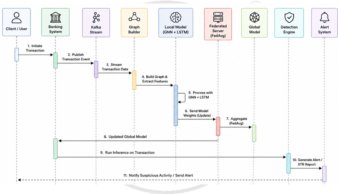
Figure 5.2: Workflow Interaction Diagram for the Proposed TBML Detection Framework
