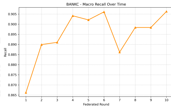
(c) BANKC Recall vs Federated Aggregation Rounds
