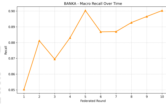
(c) BANKA Recall vs Federated Aggregation Rounds
