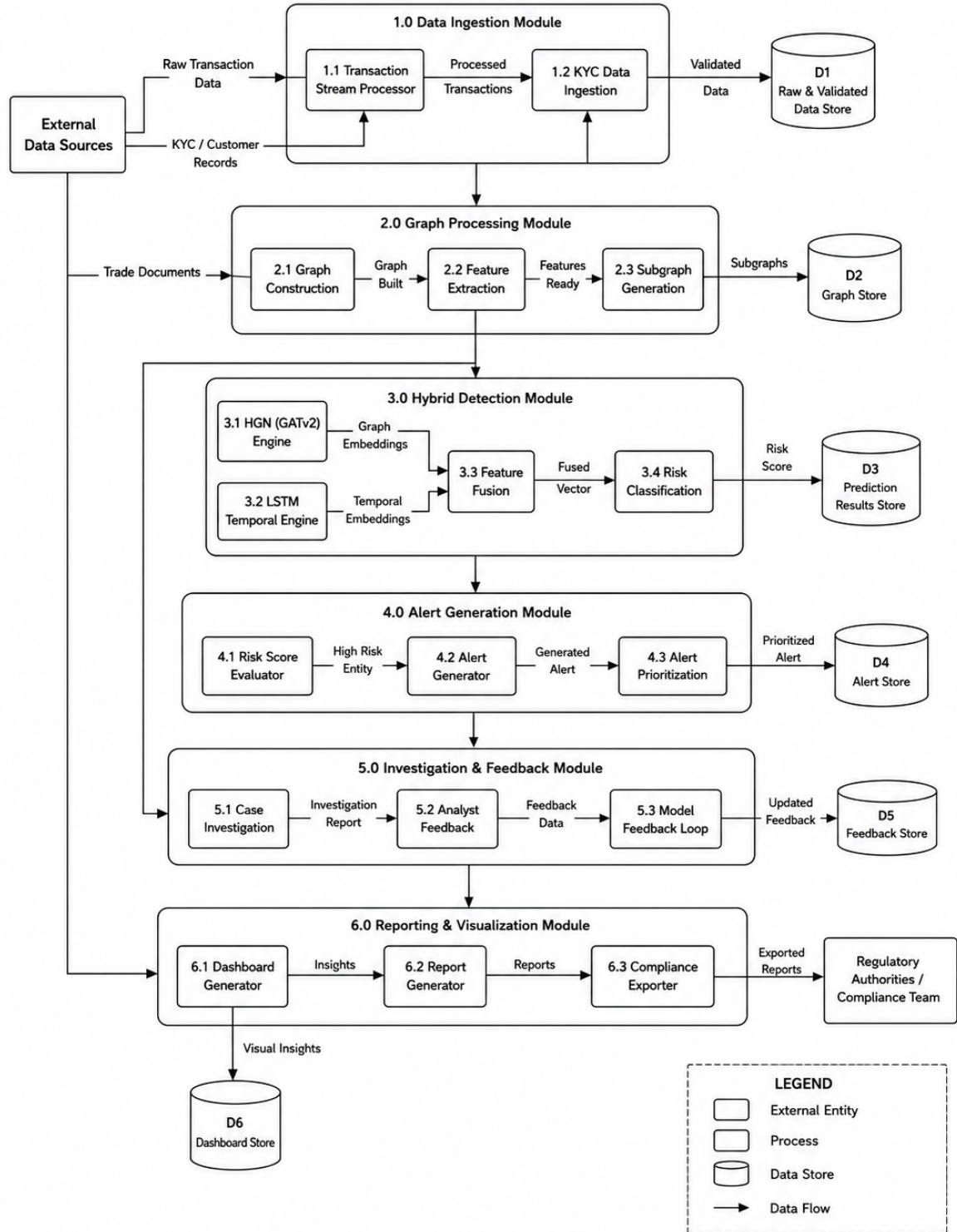
Figure 4.4: Level 2 Data Flow Diagram
