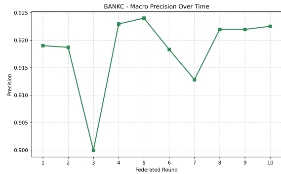
(b) BANKC Precision vs Federated Aggregation Rounds
