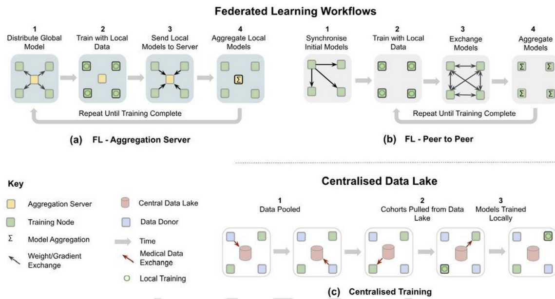
Figure 2.8: Federated Learning Workflows
