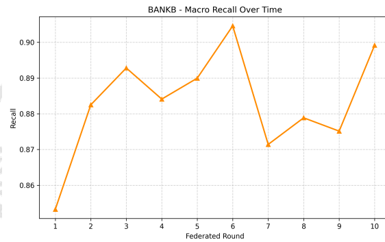
(c) BANKB Recall vs Federated Aggregation Rounds
