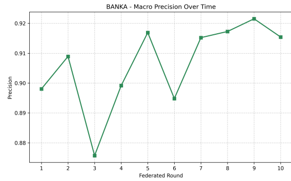
(b) BANKA Precision vs Federated Aggregation Rounds
