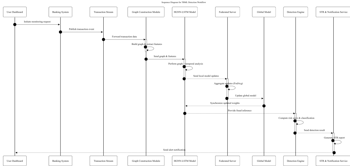
Figure 5.2: Sequence Diagram for TBML Detection Workflow
