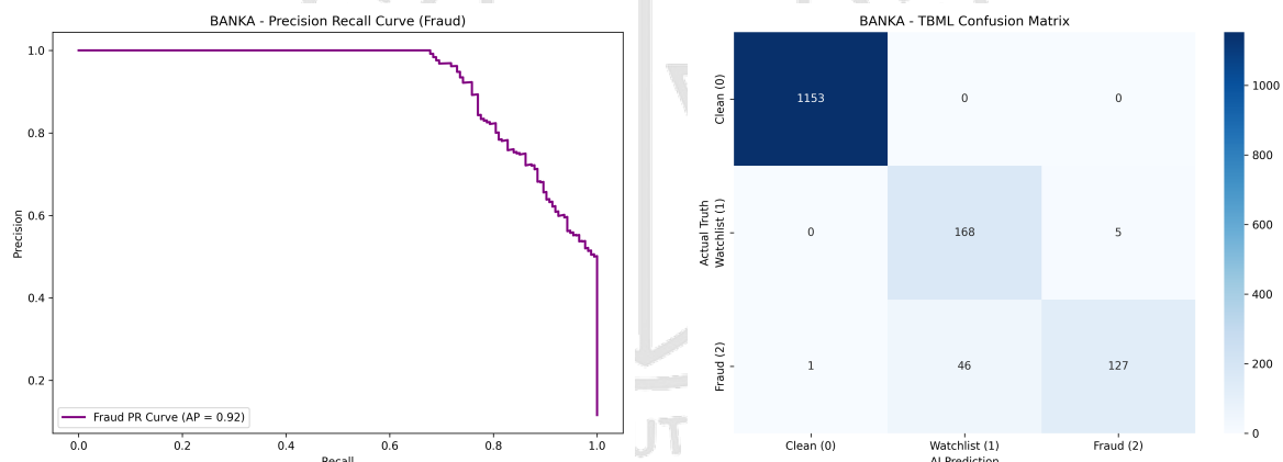
Figure 4.6: BANKA Precision–Recall Curve and Confusion Matrix Validation
