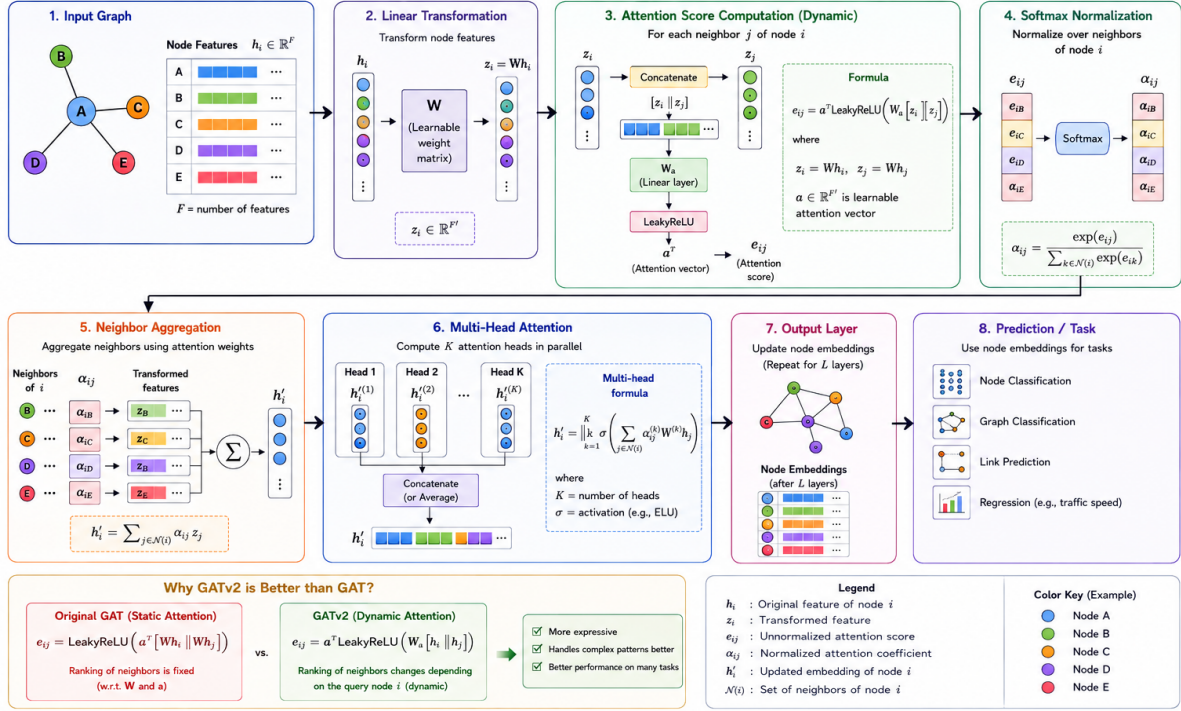
Figure 2.2: GATv2 Architecture and Working
