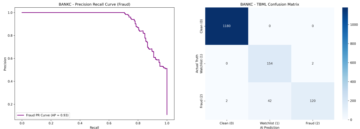
Figure 4.8: BANKC Precision–Recall Curve and Confusion Matrix Validation
