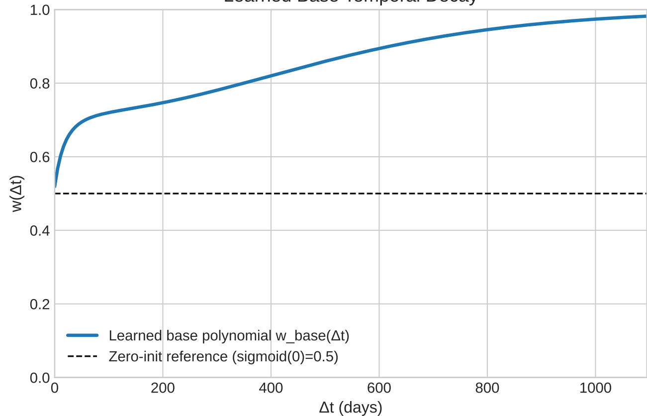
Learned Base Temporal Decay
