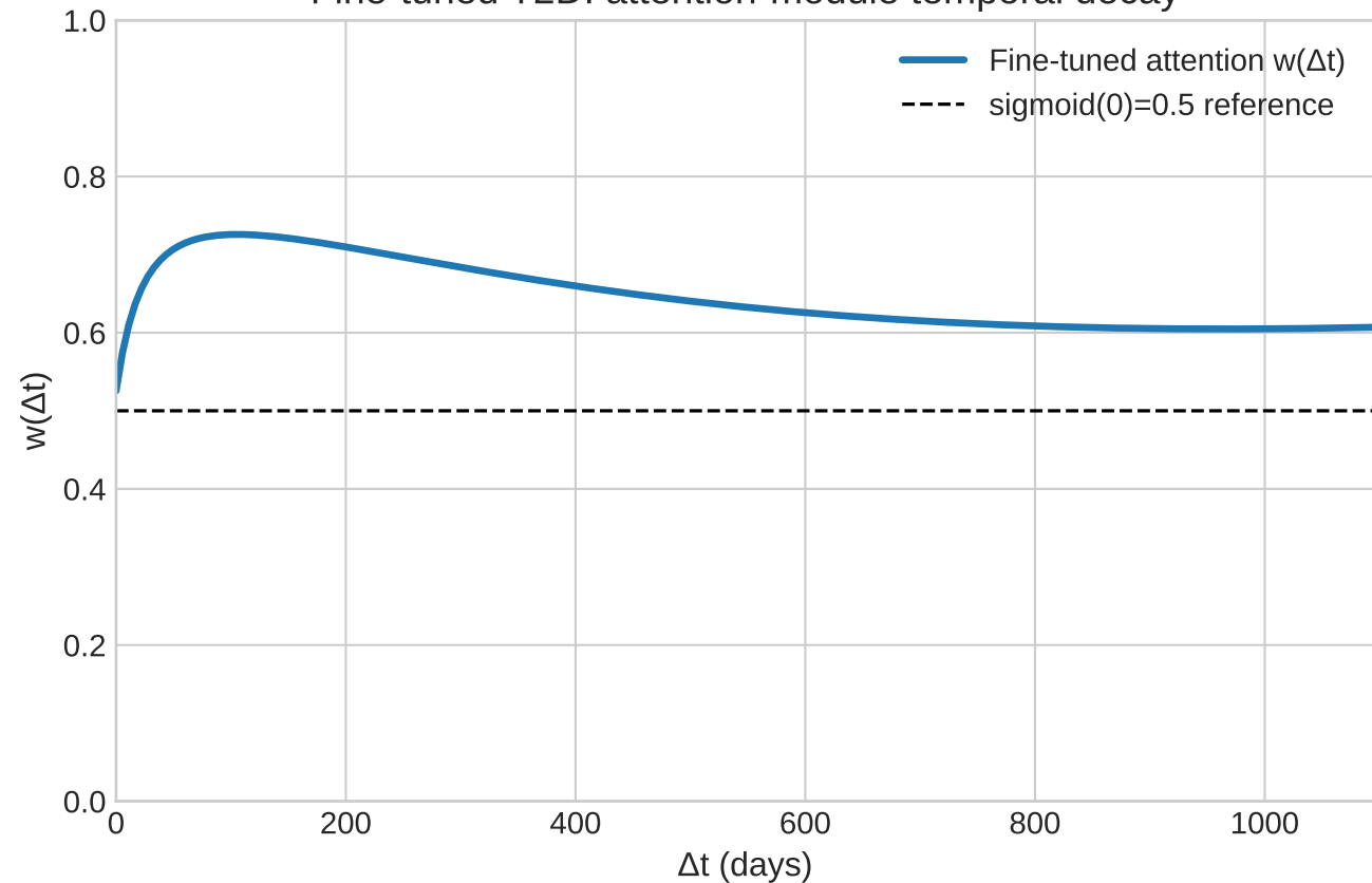
Fine-tuned T2D: attention-module temporal decay
