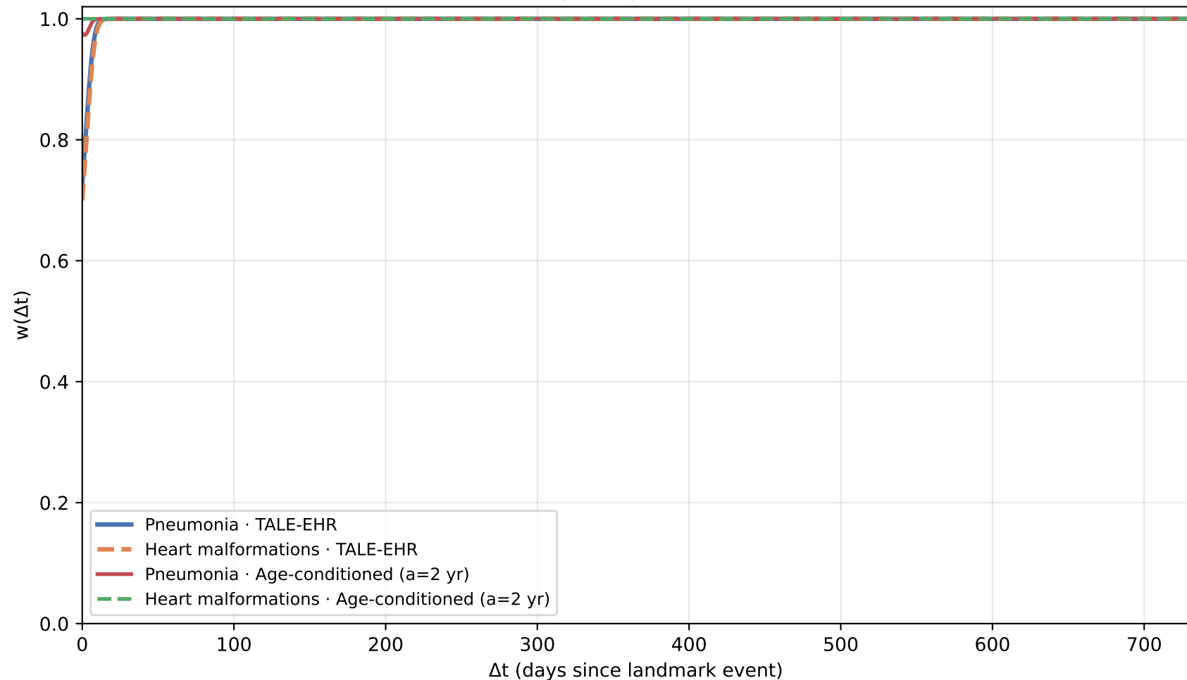
PIC fine-tuned decay comparison (attention module)
