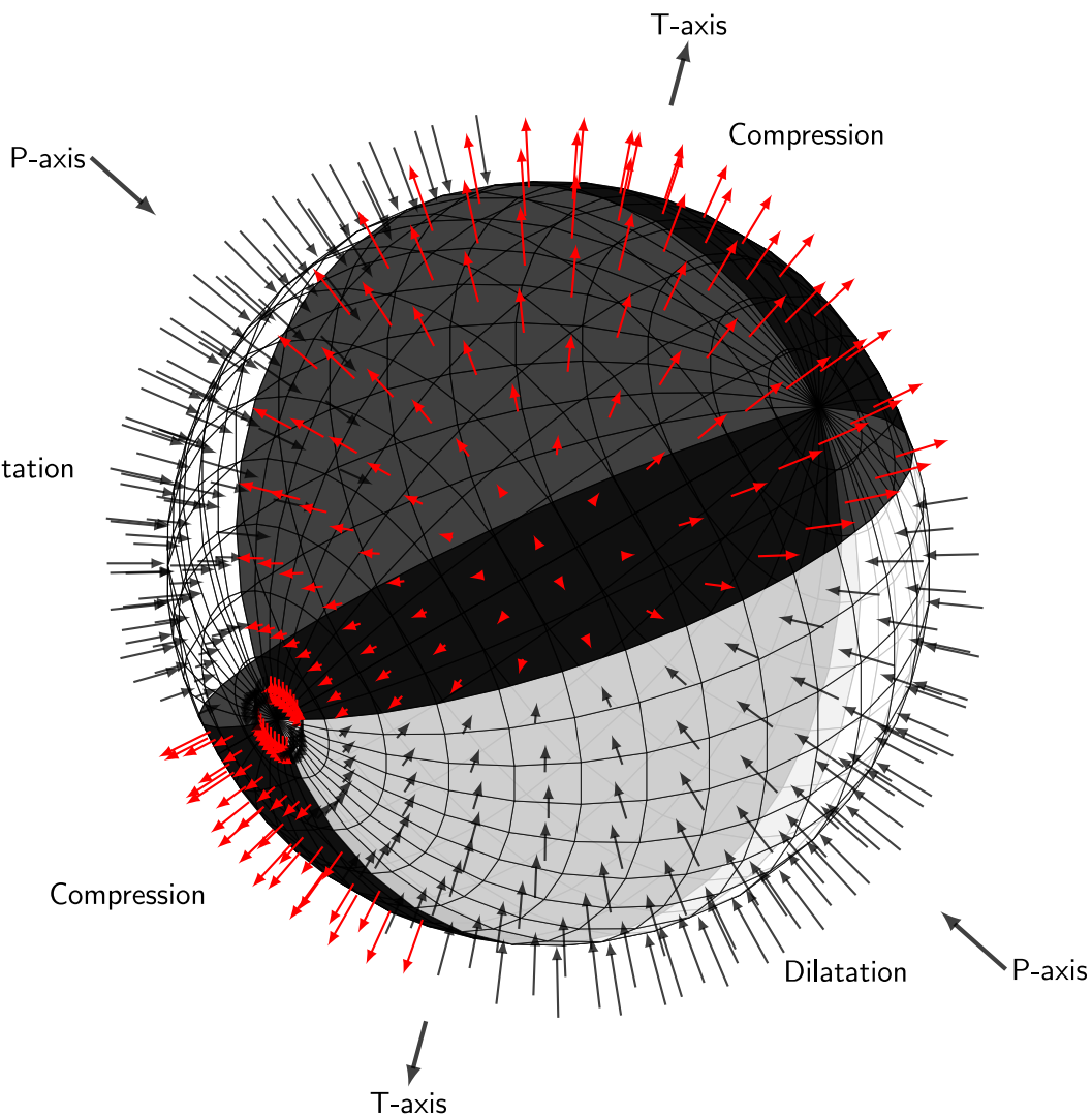
Seismic focal mechanism and Pressure-Tension axis.
