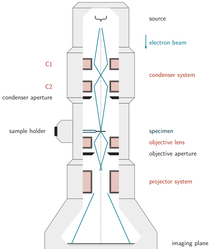
Schematic cutaway; not to scale.
