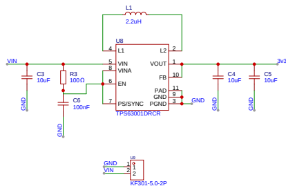
Voltage regulator
