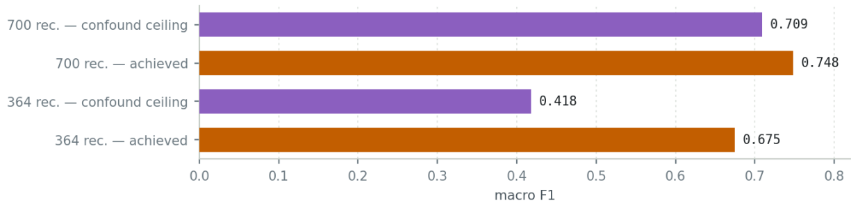
Figure 3. Margin over the confound ceiling, by scope. On the full corpus the pipeline beats the ceiling by +0.039; on the confound-free subset by +0.257 . The lower absolute score carries the greater evidential weight.
