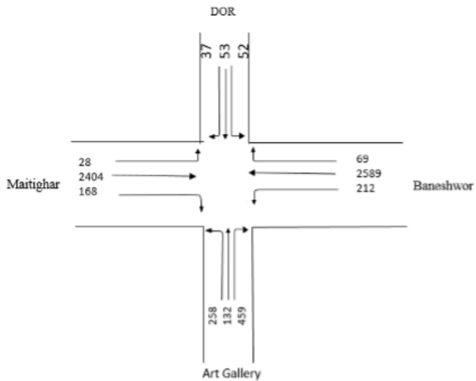
Figure C-5. Traffic Flow Diagram: Day 2 Off Peak
