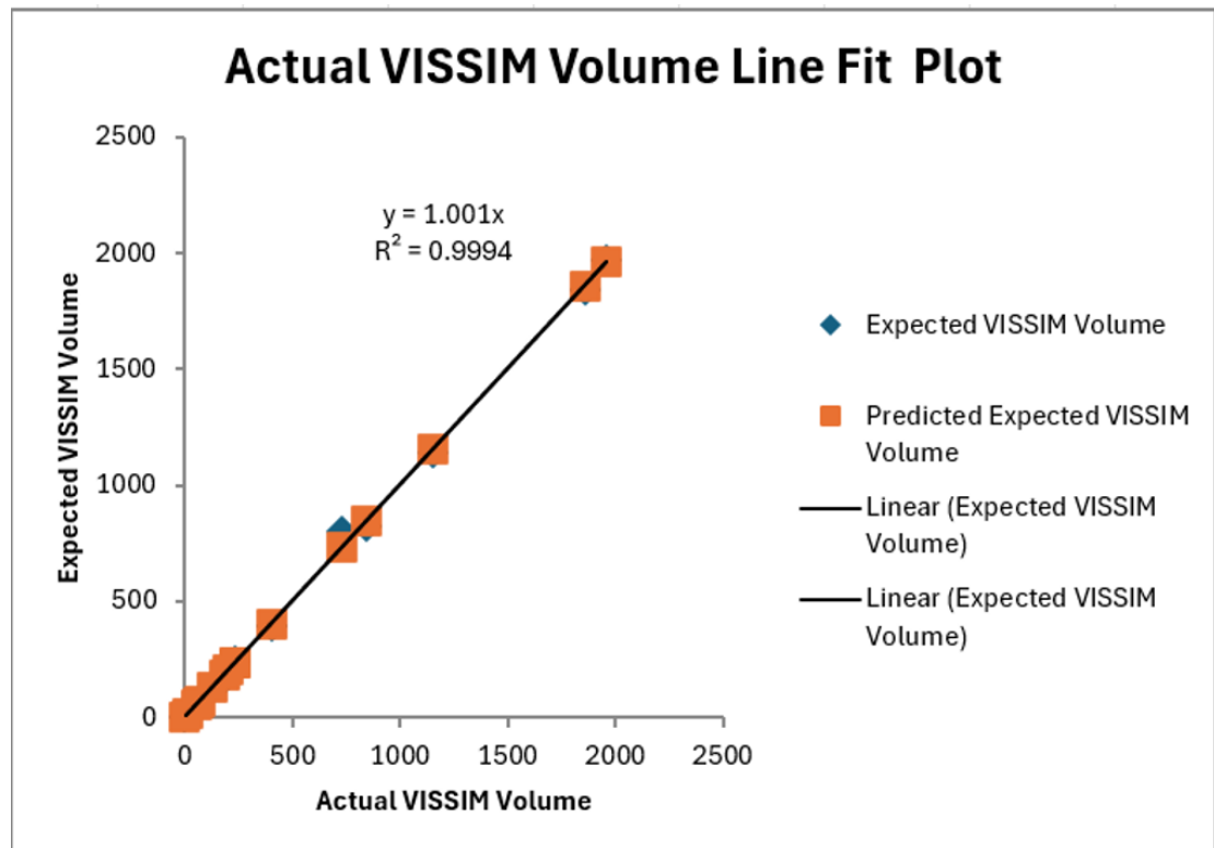
Figure 4-11. Actual VISSIM Volume Line Fit Plot
