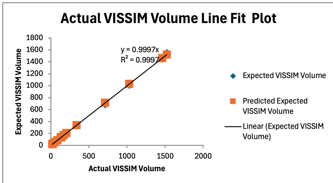
Figure 4-11. Actual VISSIM Volume Line Fit Plot
