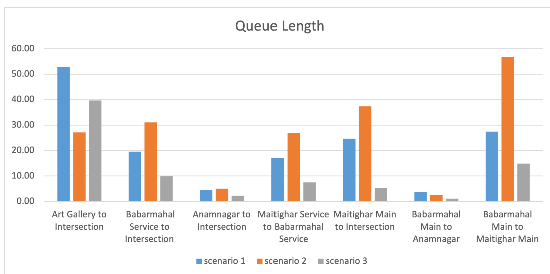
Figure B-18. Queue Length Comparison
