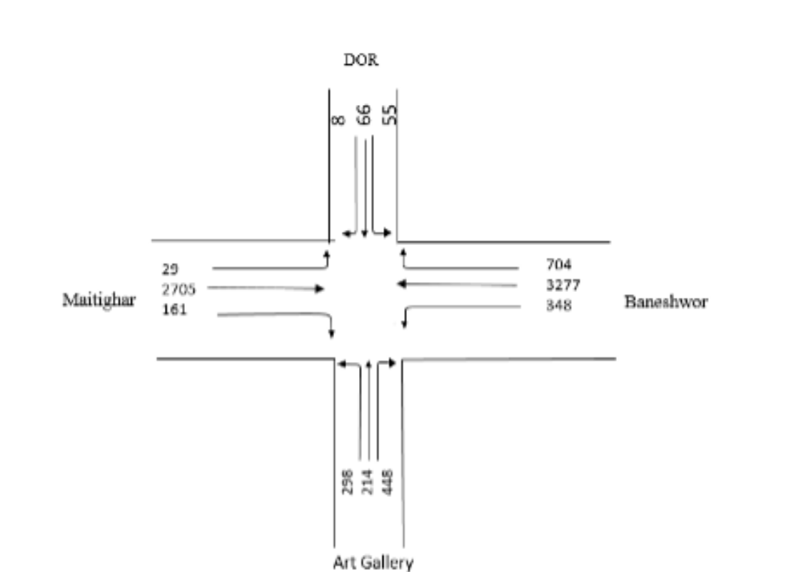
Figure C-1. Traffic Flow Diagram: Day 1 Peak
