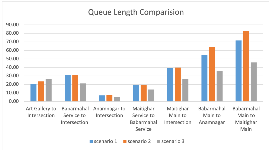
Figure B-2. Queue Length Comparision
