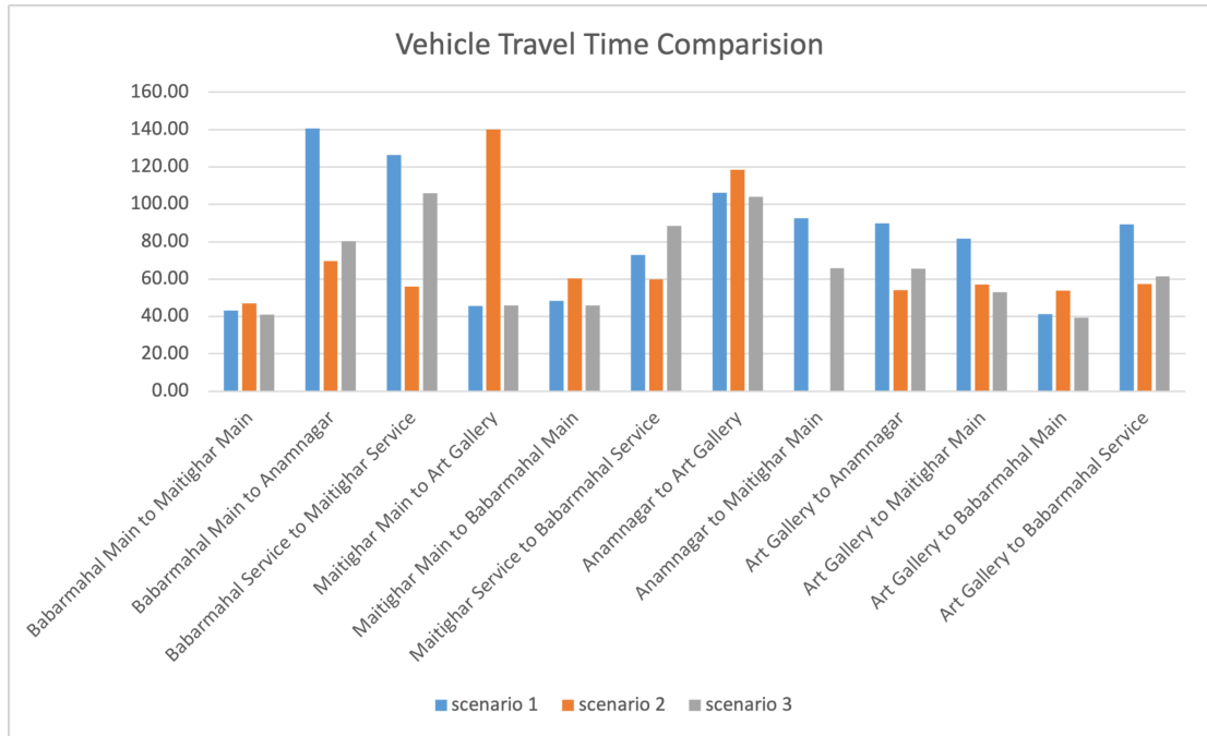
Figure B-7. Vehicle Travel Time Comparison
