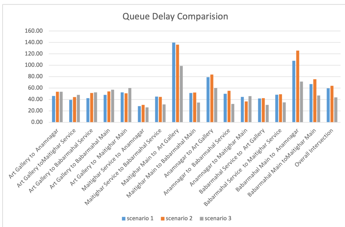
Figure B-1. Queue Delay Comparision
