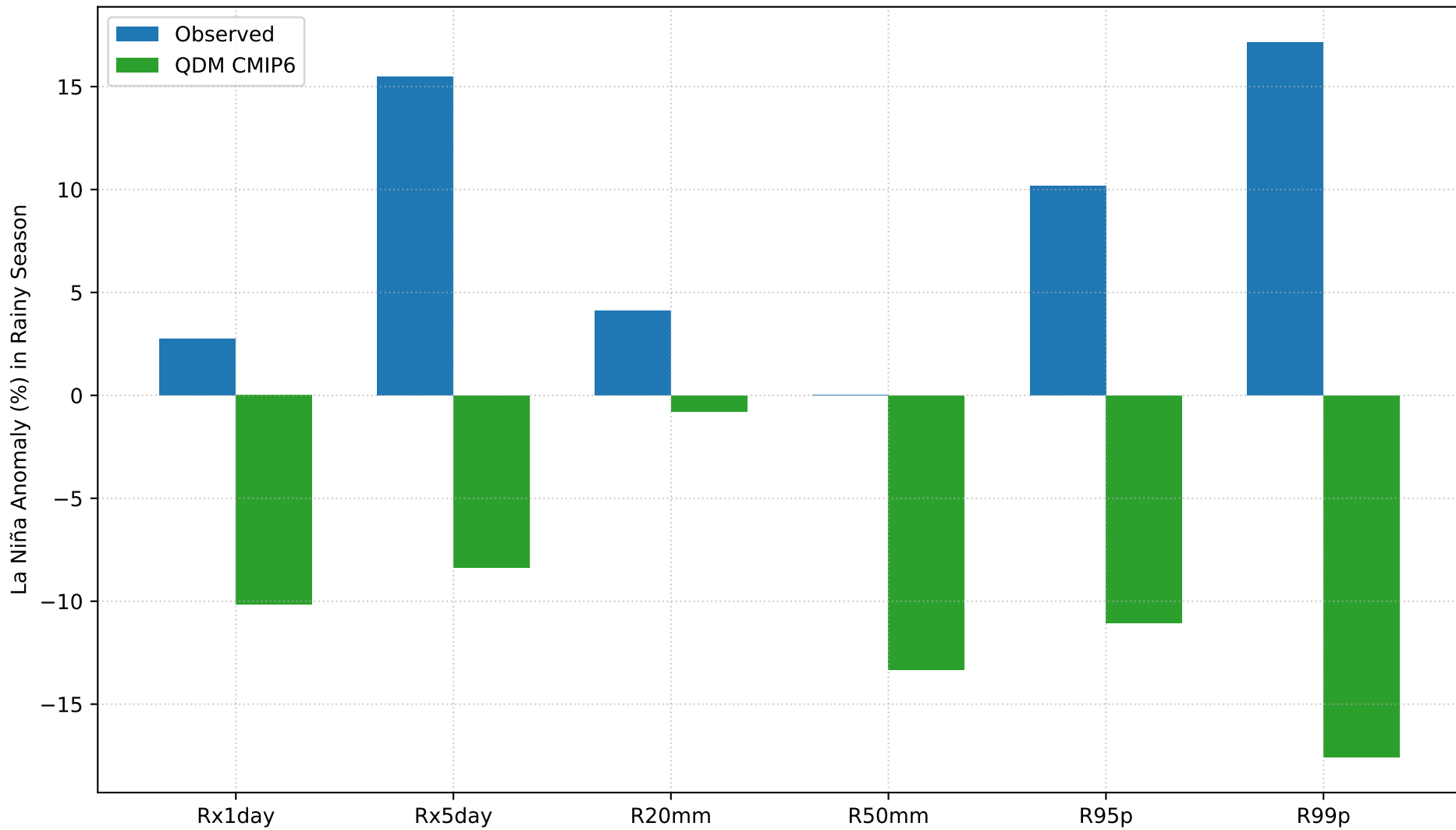
Extreme Precipitation Index Responses (Rainy Season)
