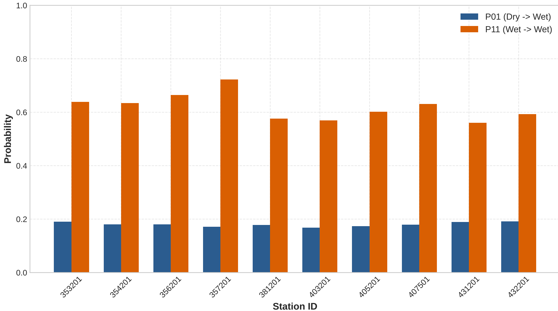
Spatial Distribution of Markov Transition Probabilities
