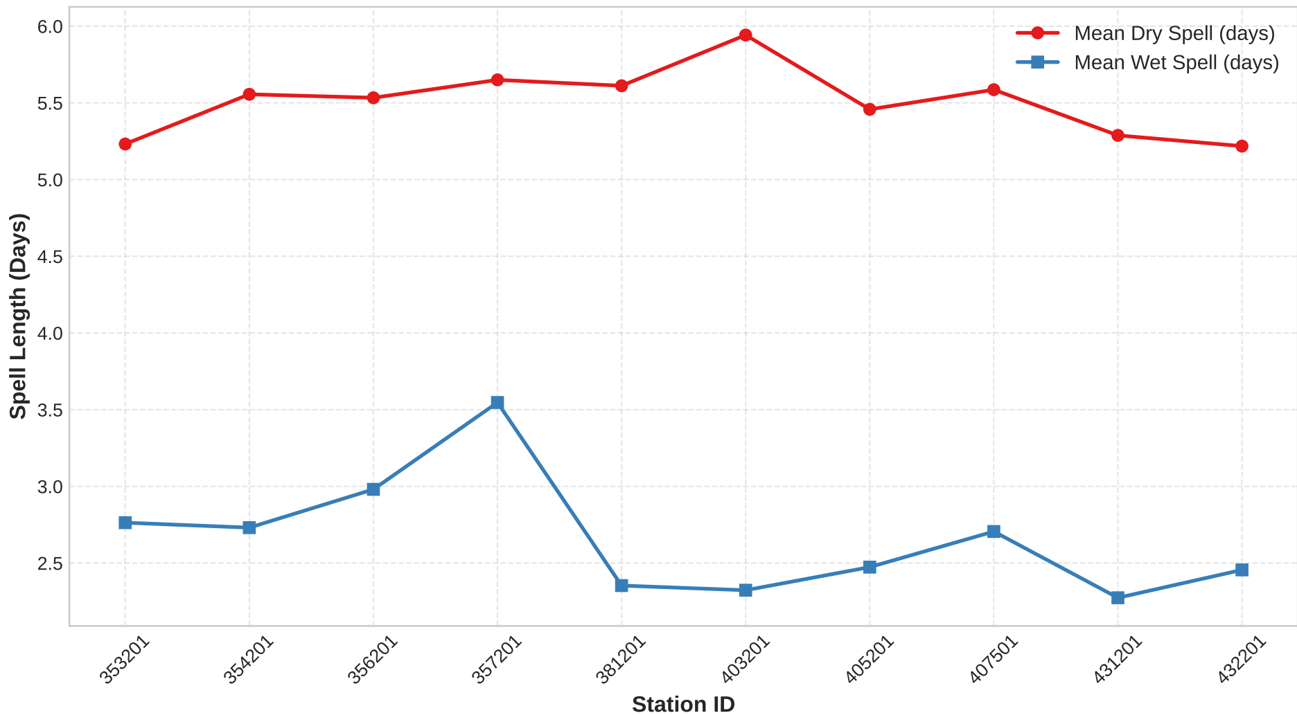
Mean Dry and Wet Spell Lengths across Stations
