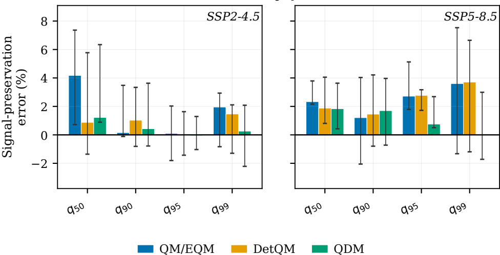
(b) wet-day quantiles
