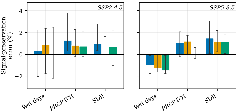
(a) bulk statistics
