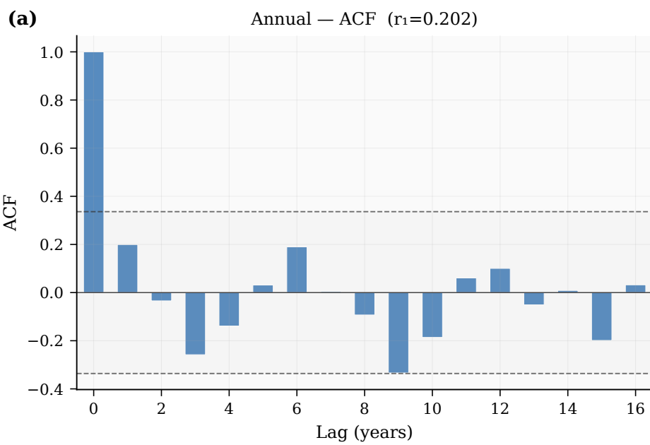
Fig. 3 — Autocorrelation structure of monsoonal rainfall series. Dashed lines: 95% significance bounds ( \pm 1.96/\sqrt{n} ).
