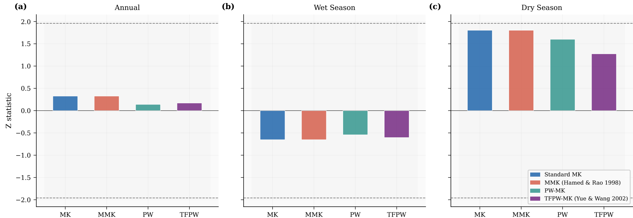
Fig. 4 — Z-statistic comparison across trend detection methods. Stars: * p < 0.05 , ** p < 0.01 , *** p < 0.001 . Dashed: \pm 1.96 critical value.
