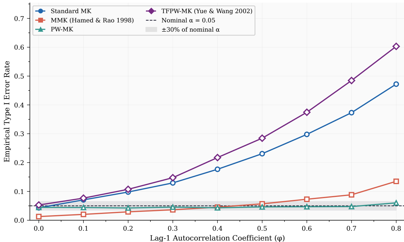
Fig. 5 — Open markers: observed Type I error. Values consistently above dashed line indicate test inflation.
