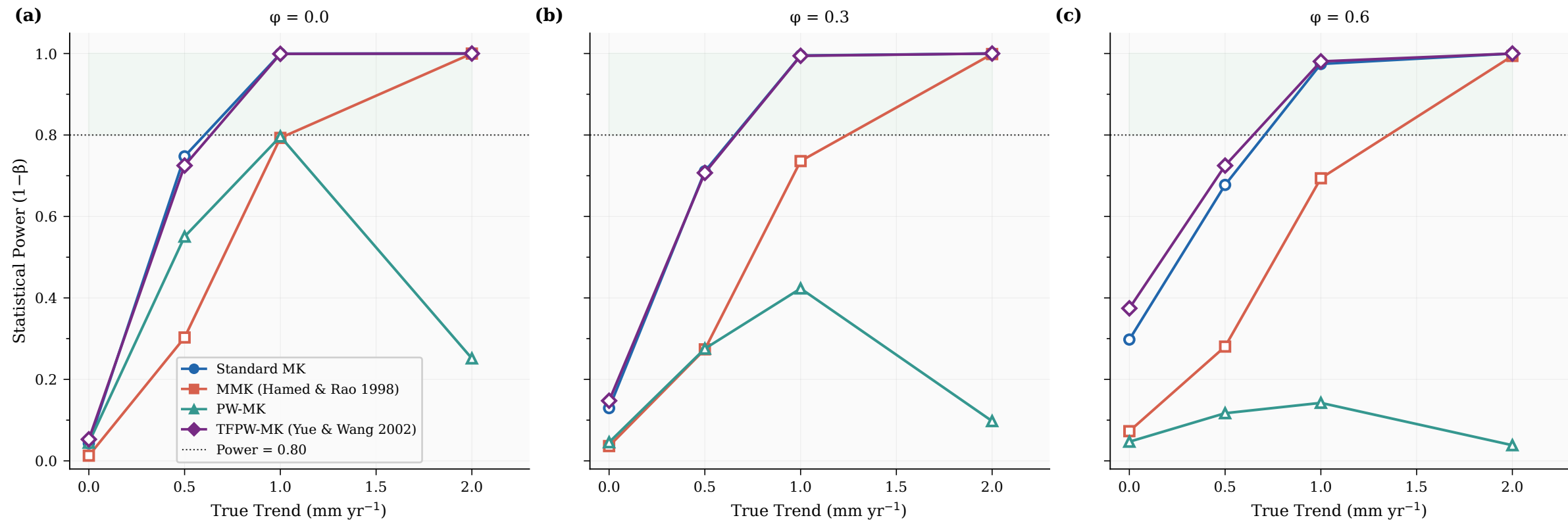
Fig. 6 — Statistical power comparison across methods and autocorrelation levels. Green shading: power \geq 0.80 .
