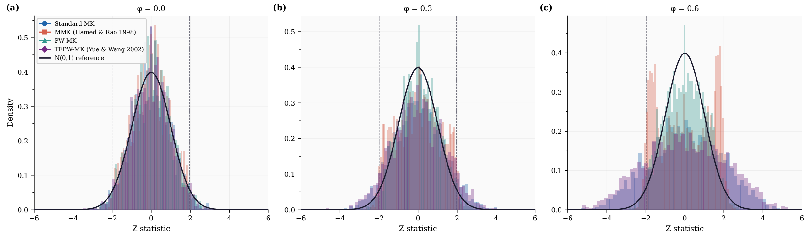
Fig. 8 — Monte Carlo Z-statistic distributions under H_0 (no trend, N = 3,000 ). Deviation from N(0,1) indicates test inflation or deflation.
