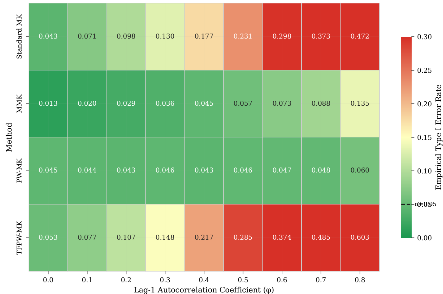
Fig. 9 — Green: near-nominal error; red: inflated Type I error.
